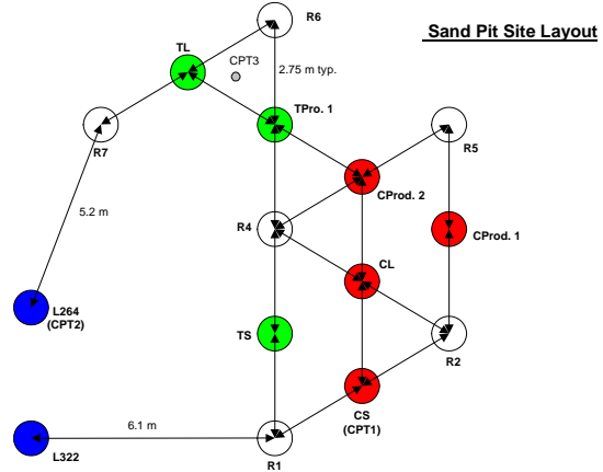
Figure 9. Typical Site Layout
